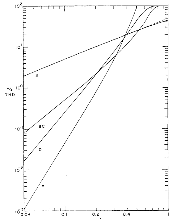
Fig. 2—Log-log plots of per cent total harmonic distortion in various cases (defined in Table III) vs the normalized distortion variable x for original square-law distortion only.
