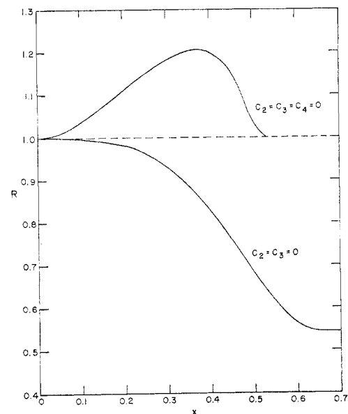
Fig. 3—Total harmonic distortion with postdistortion divided by that with predistortion vs x .
