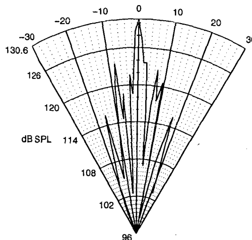
Fig. 4. Directional response of 60-kHz carrier at 3 m, measured at 1° intervals near on axis, and at larger intervals for off-axis measurements.
