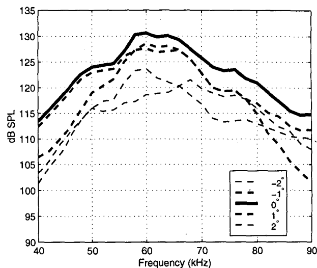
Fig. 3. Ultrasonic frequency response at 3 m for various angles, measured using pure tone bursts at 2-kHz intervals. Wide bandwidth and sharp directivity are apparent.
